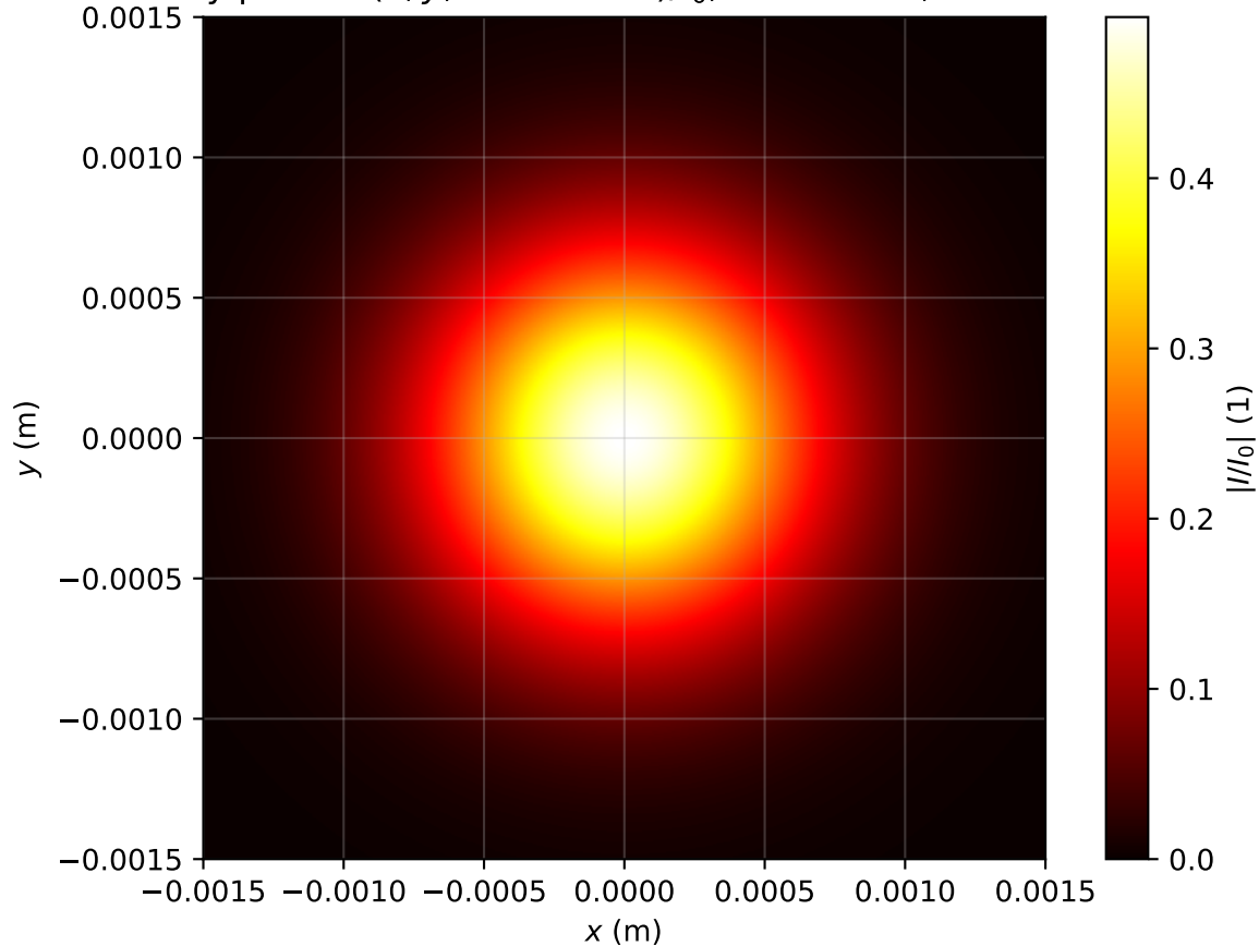
Intensity profile I(x, y, z = 2.388m)/I_0 , P_{in}=0.2P_{cr} , artificial time
